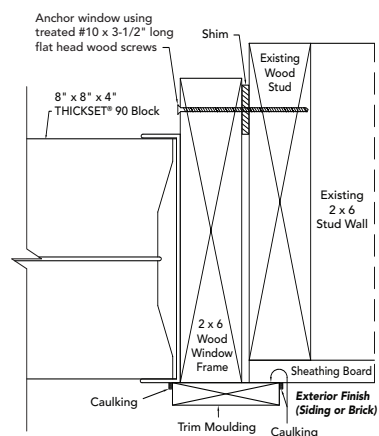
Wood Framing Wall Detail
