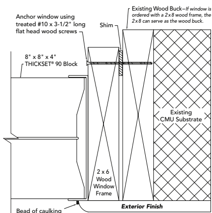
CMU Wall Detail
